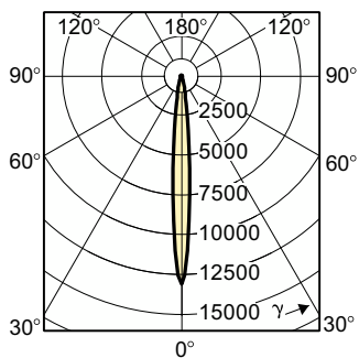
Light Distribution Diagram - Brill 50W GU5.3 12V 10D 1CT/10X5F
