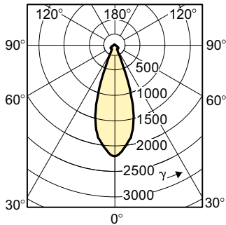
Light Distribution Diagram - EXN 50W GU5.3 12V MR16 36D CL 1CT/10X5F
