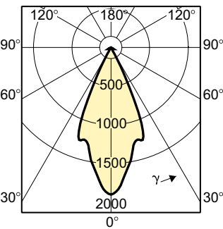
Light Distribution Diagram - MASTERLine 111 45W G53 12V 45D 1CT/6
