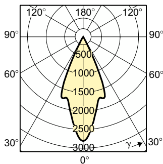
Light Distribution Diagram – MASTERLine 111 60W G53 12V 45D 1CT/6
