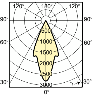
Light Distribution Diagram - MASTERLine 111 60W G53 12V 45D 1CT/6
