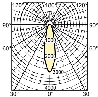
Light Distribution Diagram - HalogenA PAR30S 100W E27 230V 30D 1CT/15
