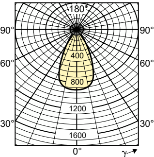
Light Distribution Diagram - PAR20 HAL 50W E27 120V 25D 1CT/15
