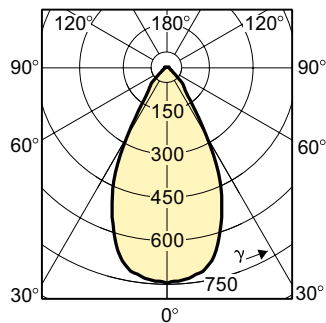
Light Distribution Diagram - MASTERL ES 30W GU5.3 12V 60D 1CT/4X5F
