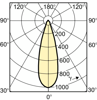
Light Distribution Diagram - EnAdvIR Alu 20W 12V MR16 36D 1CT/4XF5
