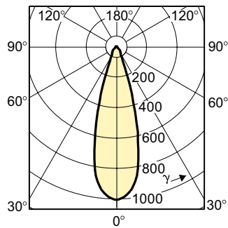
Light Distribution Diagram - EnAdvIR Alu 20W 12V MR16 36D 1CT/4XF5
