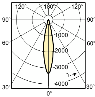
Light Distribution Diagram - 30MRC16/IRC/ALU/NFL24 20PK
