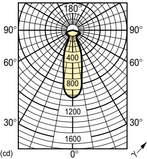
Light Distribution Diagram - Ref 60W E27 230V NR63 30D FR 1CT/30
