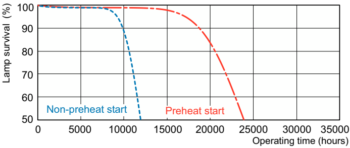
Life Expectancy Diagram - F28T5/835 ALTO TG 40PK
