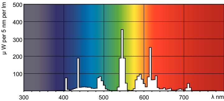
Spectral Power Distribution Colour - F28T5/835 ALTO TG 40PK
