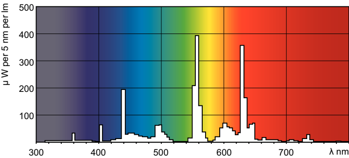
Spectral Power Distribution Colour - F54T5/841/HO/EA/ALTO TG 49W
