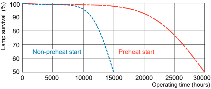
Life Expectancy Diagram - F54T5/841/HO/EA/ALTO TG 49W
