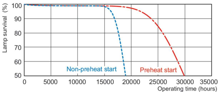
Life Expectancy Diagram - F54T5/841/HO/EA/ALTO TG 49W
