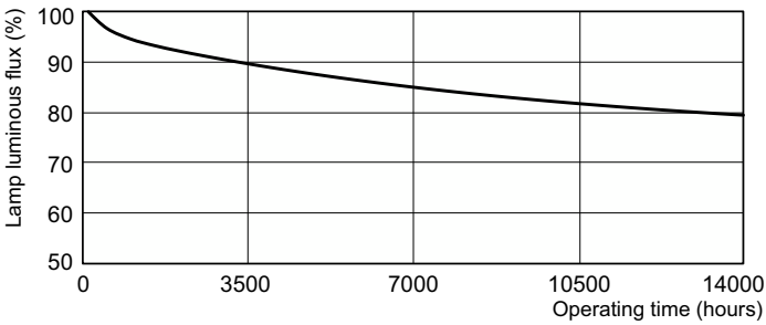
Lumen Maintenance Diagram - MASTER PL-C 10W/865/2P 1CT/5X10BOX
