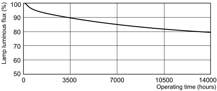
Lumen Maintenance Diagram - PL-C 13W/827/2P/ALTO 10PK
