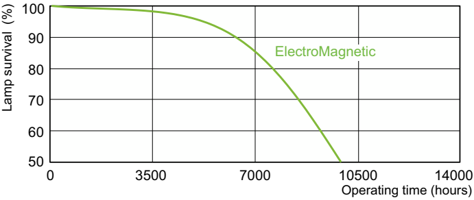
Life Expectancy Diagram - PL-C 18W/830/2P/ALTO 10PK
