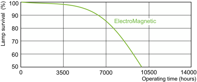
Life Expectancy Diagram - MASTER PL-C 26W/830/2P 1CT/5X10CC
