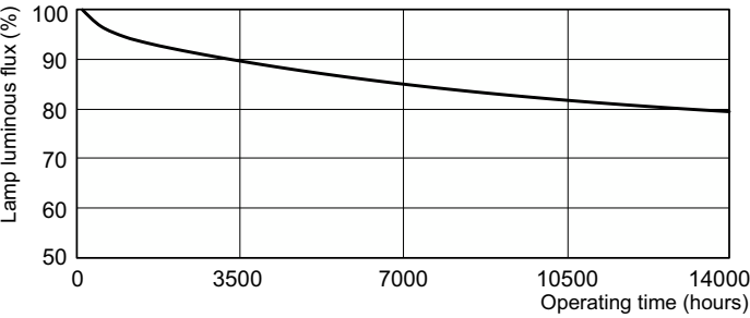
Lumen Maintenance Diagram - PL-C26W/830/2P/ALTO 10PK
