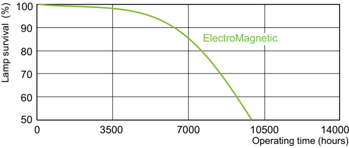
Life Expectancy Diagram - PL-C26W/830/2P/ALTO 10PK
