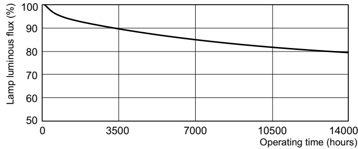
Lumen Maintenance Diagram - PL-C 26W/841/2P/ALTO 10PK
