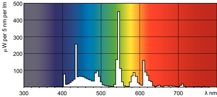
Spectral Power Distribution Colour - MASTER PL-C 26W/865/2P 1CT/5X10CC
