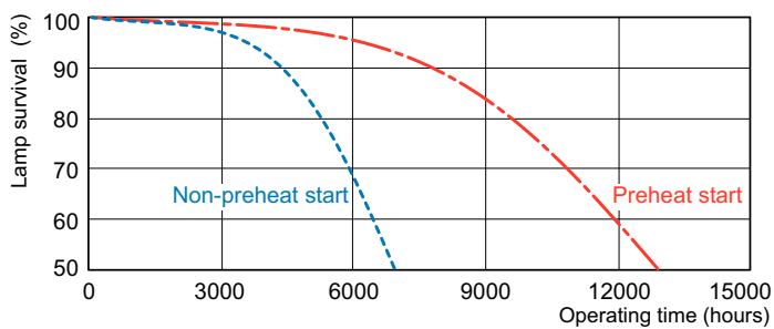
Life Expectancy Diagram - PL-C 26W/827/XEW/4P/ALTO 21W
