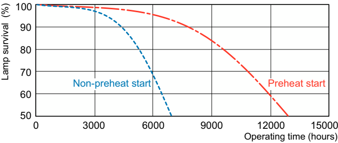
Life Expectancy Diagram - PL-C 13W/830/4P/ALTO 10PK
