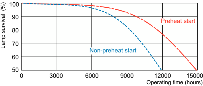
Life Expectancy Diagram - MASTER PL-C 18W/865/4P 1CT/5X10BOX
