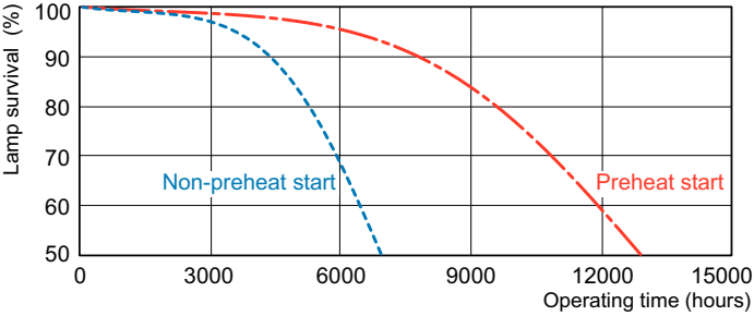
Life Expectancy Diagram - MASTER PL-C 18W/865/4P 1CT/5X10CC
