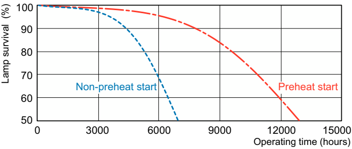
Life Expectancy Diagram - PL-C 26W/840/4P 1CT/5X10BOX
