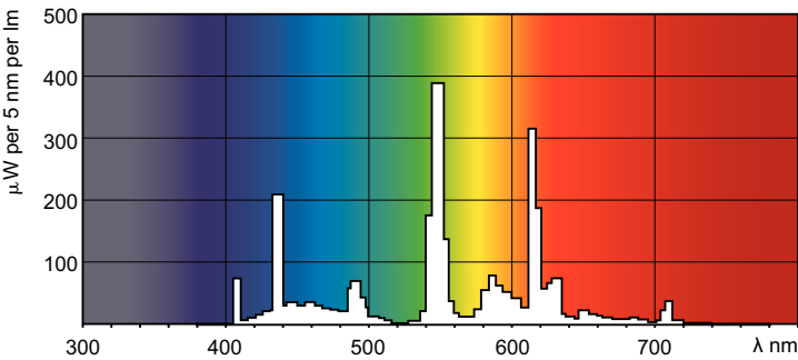
Spectral Power Distribution Colour - MASTER PL-C 26W/840/4P 1CT/5X10CC
