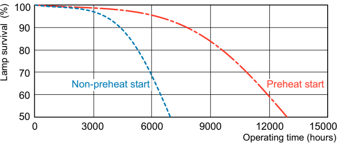
Life Expectancy Diagram - PL-T 26W/841/A/4P 1CT/5X10BOX ALTO
