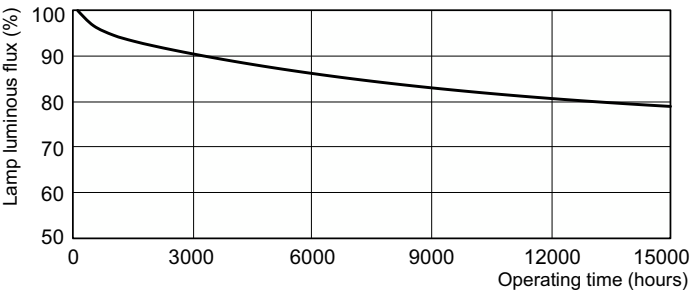
Lumen Maintenance Diagram - PL-T 26W/841/A/4P 1CT/5X10BOX ALTO
