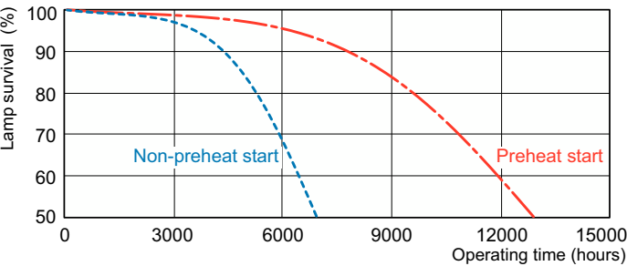
Life Expectancy Diagram - PL-T 32W/835/A/4P 1CT/5X10BOX ALTO
