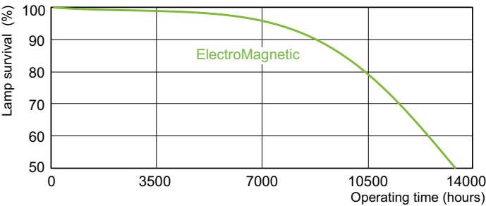
Life Expectancy Diagram - MASTER PL-T 26W/840/2P 1CT/5X10BOX
