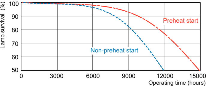
Life Expectancy Diagram - MASTER PL-T 32W/830/4P 1CT/5X10BOX
