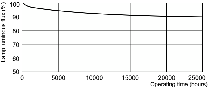
Lumen Maintenance Diagram - MASTER TL-D Secura 18W/830 SLV/25
