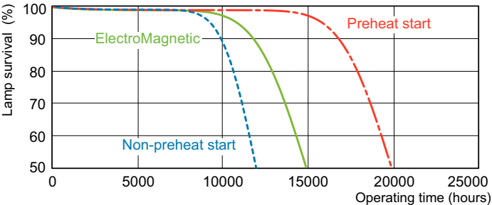
Life Expectancy Diagram - MASTER TL-D Secura 18W/830 SLV/25
