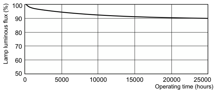
Lumen Maintenance Diagram - MASTER TL-D Secura 36W/830 SLV/25
