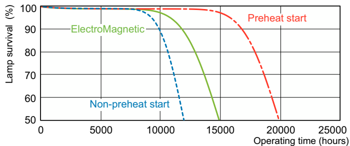
Life Expectancy Diagram - MASTER TL-D Secura 36W/830 SLV/25
