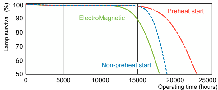
Life Expectancy Diagram - MASTER TL-D Secura 36W/830 SLV/25
