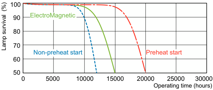
Life Expectancy Diagram - TL-D 58W/865 1PP/10
