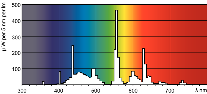
Spectral Power Distribution Colour - TL-D 58W/865 1PP/10
