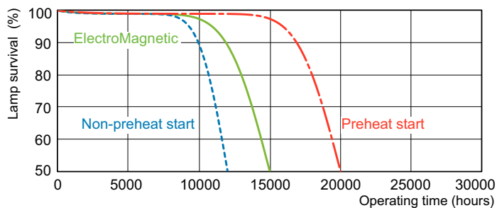
Life Expectancy Diagram - MASTER TL-D Super 80 23W/865 1SL/25
