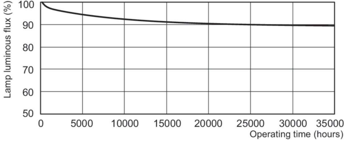
Lumen Maintenance Diagram - MASTER TL5 HE 14W/865 SLV/40
