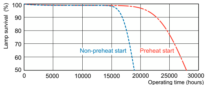
Life Expectancy Diagram - MASTER TL5 HE Secura 14W/840 UNP/40
