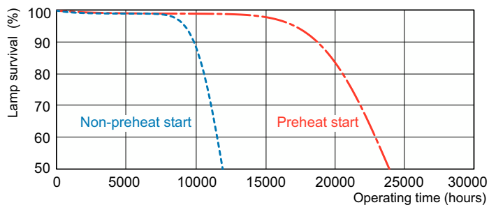
Life Expectancy Diagram - MASTER TL5 HE Secura 14W/840 UNP/40
