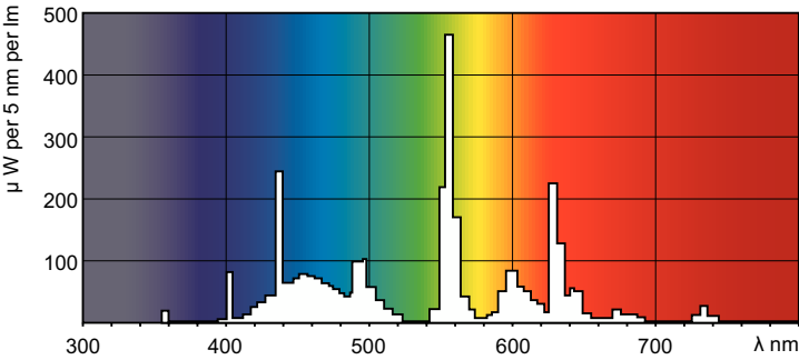
Spectral Power Distribution Colour - MASTER TL5 HE 21W/865 UNP/40
