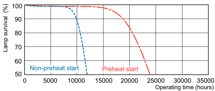
Life Expectancy Diagram - TL5 HE 28W WW 1PP/10
