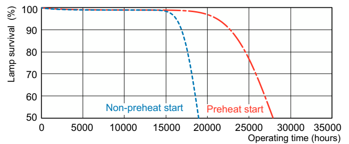
Life Expectancy Diagram - TL5 HE 28W WW 1PP/10
