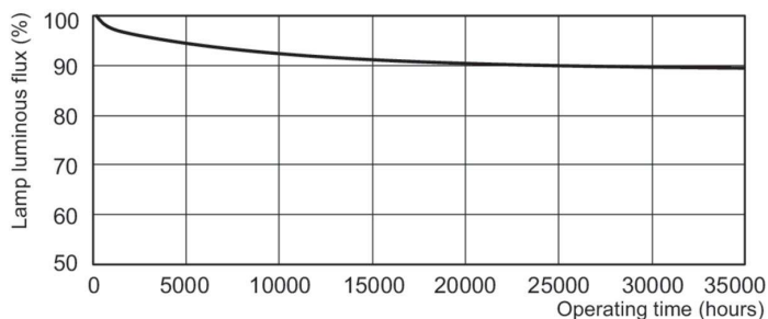
Lumen Maintenance Diagram - MASTER TL5 HE 28W/865 SLV/40
