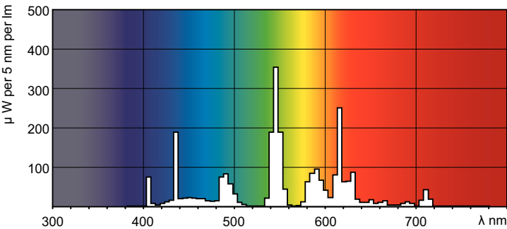
Spectral Power Distribution Colour - MASTER TL5 HE 35W/835 SLV/40
