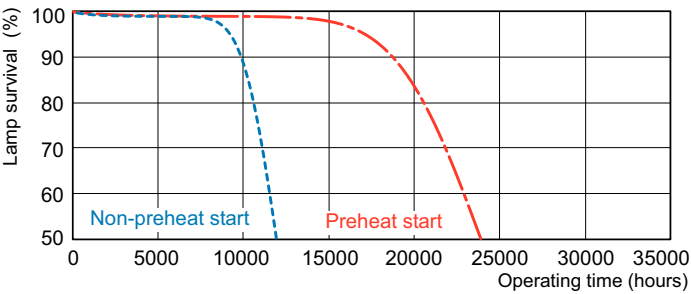
Life Expectancy Diagram - MASTER TL5 HE 35W/835 SLV/40
