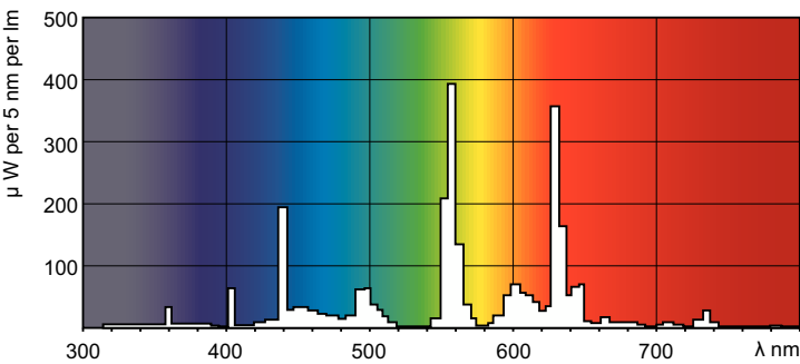
Spectral Power Distribution Colour - MASTER TL5 HE Secura 35W/840 UNP/40
