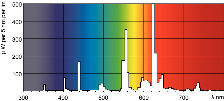
Spectral Power Distribution Colour - MASTER TL5 HO 49W/827 SLV/40
