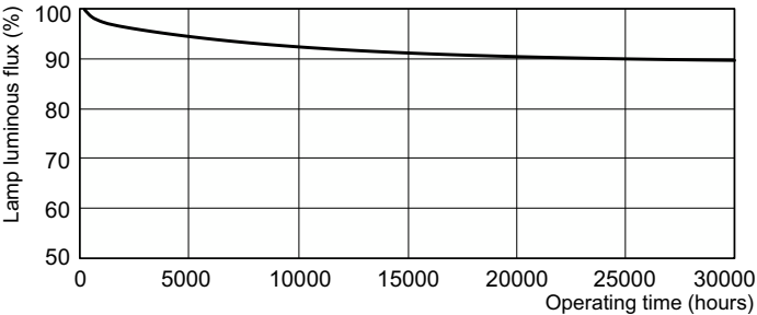
Lumen Maintenance Diagram - MASTER TL5 HO 49W/865 UNP/40
