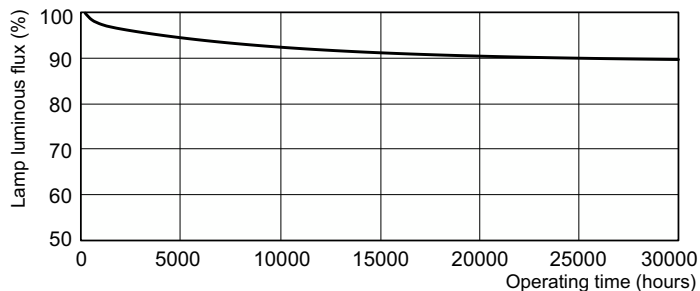
Lumen Maintenance Diagram - MASTER TL5 HO 49W/865 SLV/40
