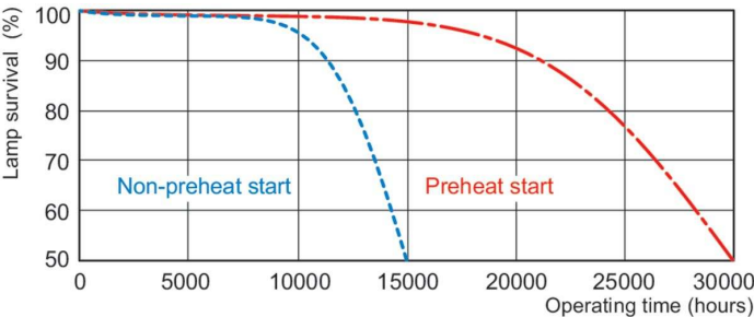
Life Expectancy Diagram - MASTER TL5 HO 39W/830 UNP/40
