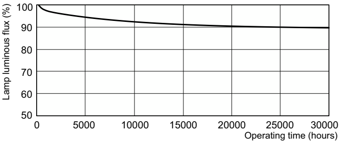
Lumen Maintenance Diagram - MASTER TL5 HO 39W/830 UNP/40
