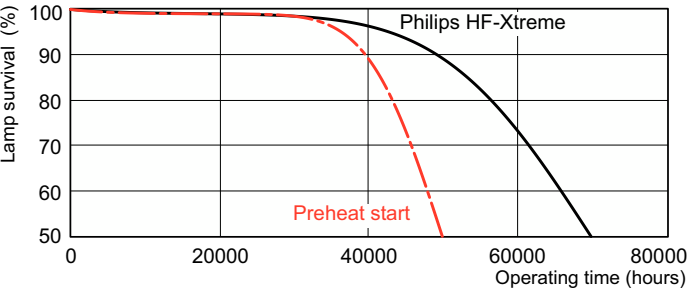
Life Expectancy Diagram - F54T5/TL830/HO/XXL 40 PK
