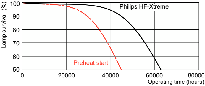
Life Expectancy Diagram - F54T5/TL830/HO/XXL 40 PK
