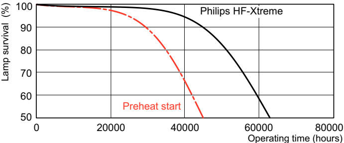
Life Expectancy Diagram - MASTER TL5 HO Xtra 54W/830 SLV/20
